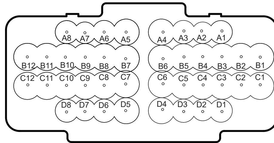
CONN1 ENG/REAR H-TO-H CONN (M)
